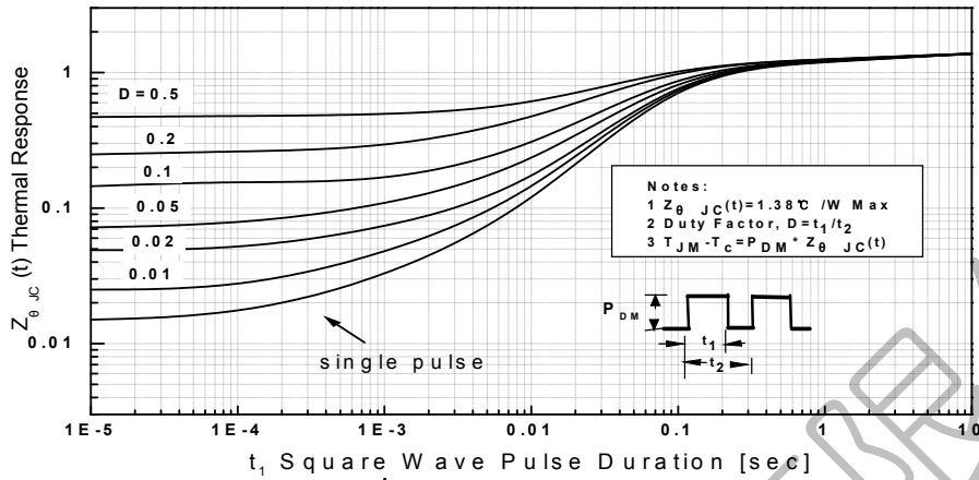
Transient Thermal Response Curve For JCS5N50CC
