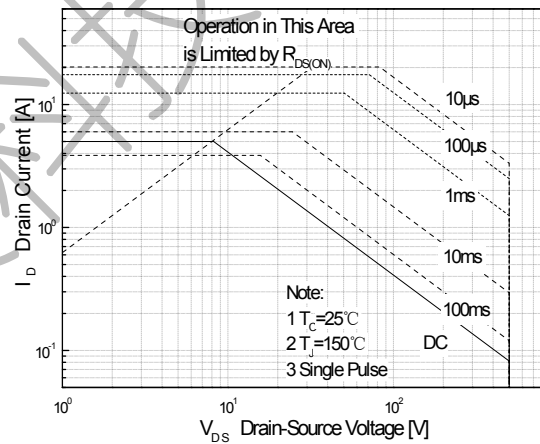
Maximum Safe Operating Area For JCS5N50FC
